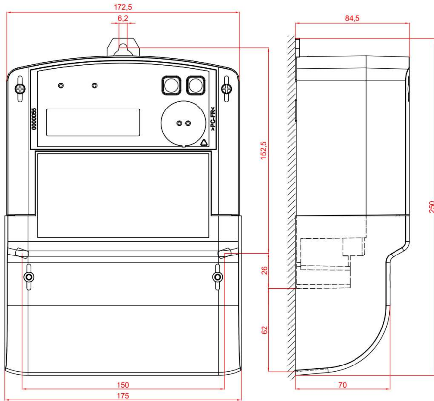
Figure 2.2. Dimensions of the meter
