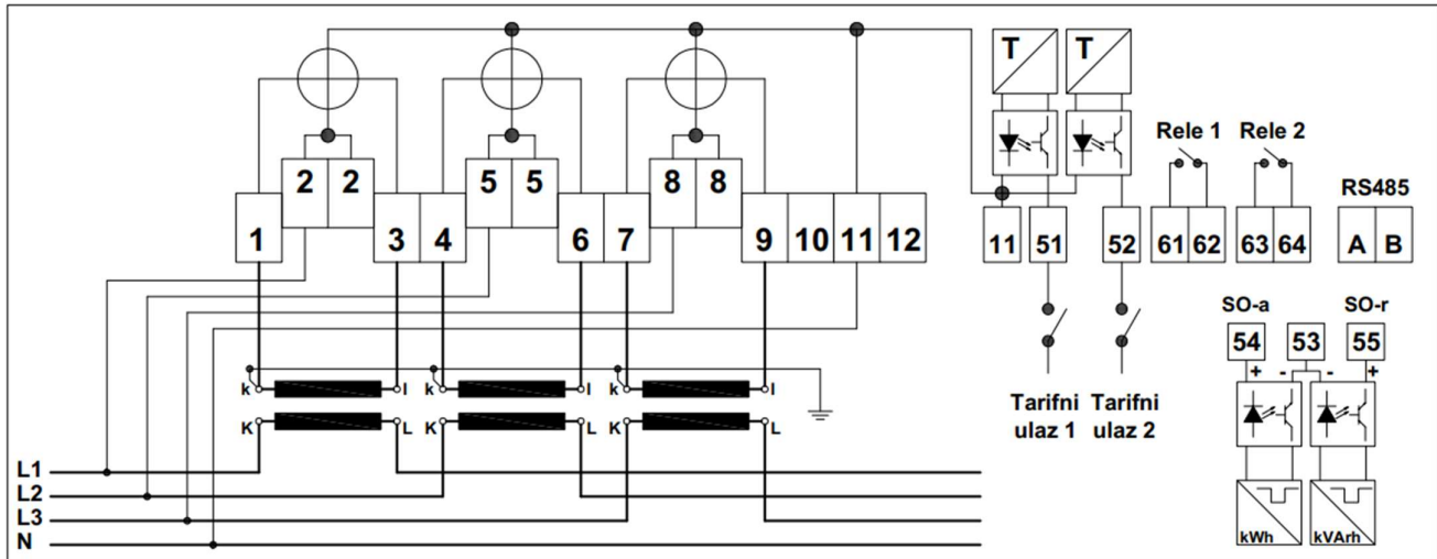
Figure 2.7 Current transformer operated meter connection scheme
